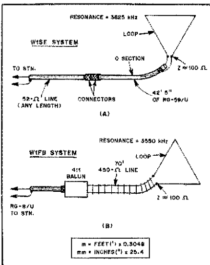
Fig. 3 — At A is the feed method used at WISE. A coaxial Q section closely matches the 100-ohm feed impedance to a 52-ohm coaxial line. Illustration B shows the W1FB feed arrangement. Open-wire line, a balun transformer and a short length of RG-8/U cable permit multiband use with a Transmatch. Ideally, the open-wire line would continue all the way to the Transmatch, and the balun transformer would be located at the Transmatch.
